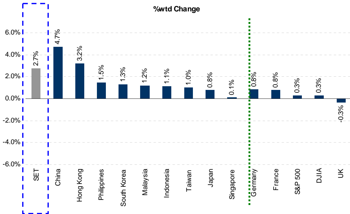
รูป a Global Indices Return : 30 MAR – 3 APR 2015
